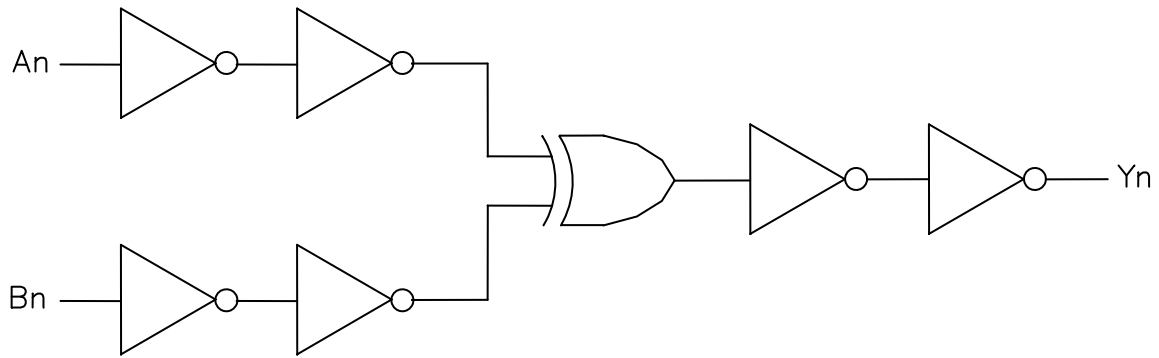
FIGURE 3. Logic diagram.
