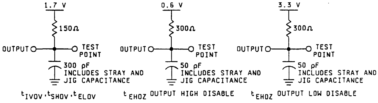
FIGURE 4. Timing waveform and test circuit.
