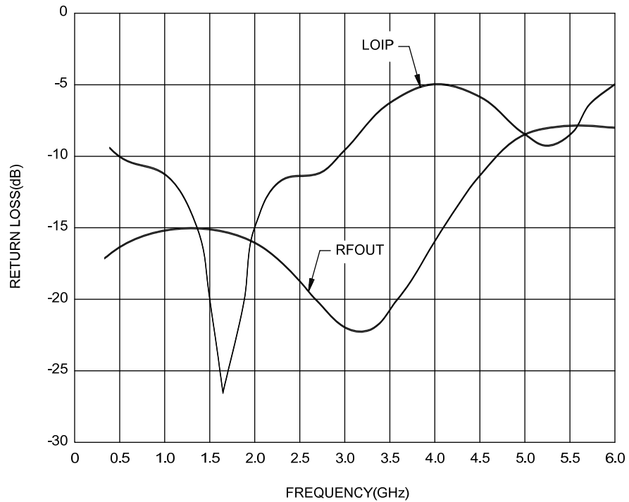
FIGURE 5. Return Loss of LOIP (LOIN AC-Coupled to Ground) S11 and RFOUT S22 from 450 MHz to 6000 MHz.
