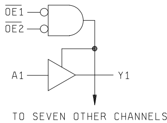
FIGURE 3. Logic diagram.
