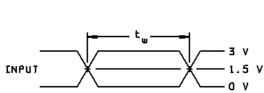
VOLTAGE WAVEFORMS PULSE DURATION
