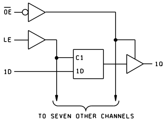
FIGURE 3. Logic diagram.
