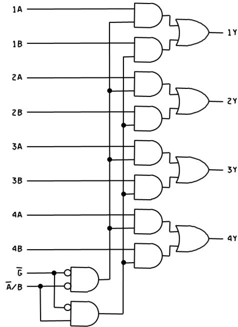
FIGURE 3. Logic diagram.
