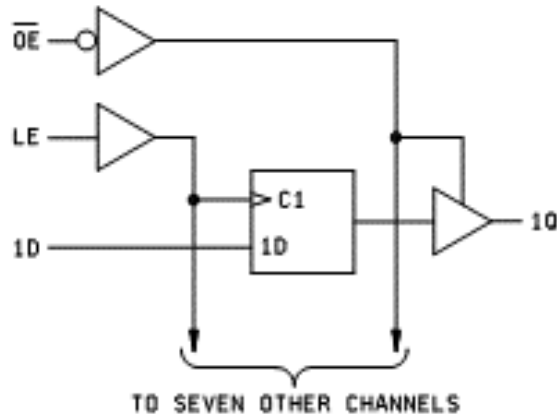
FIGURE 3. Logic diagram.
