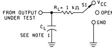
LOAD CIRCUIT FOR 3-STATE AND OPEN-DRAIN OUTPUTS
