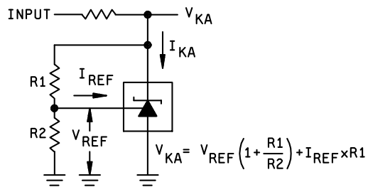
CIRCUIT B FOR V_{KA} > V_{REF}
