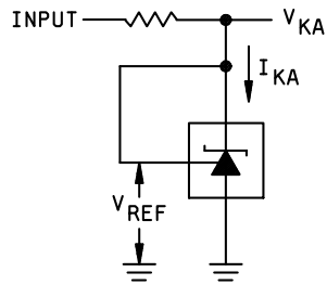
CIRCUIT A FOR V_{KA} = V_{REF}
