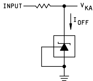
CIRCUIT C FOR I_{OFF}
