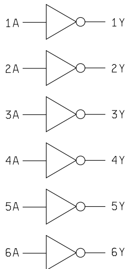
FIGURE 2. Logic diagram.
