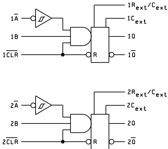
FIGURE 3. Logic diagram.
