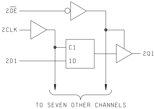
FIGURE 3. Logic diagram.
