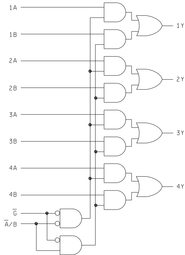
FIGURE 3. Logic diagram.
