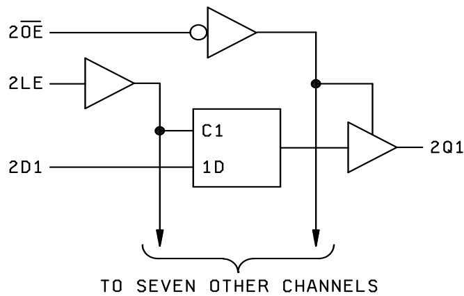
FIGURE 3. Logic diagram.
