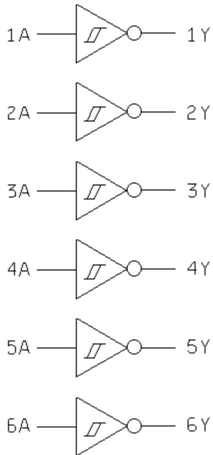
FIGURE 3. Logic diagram.
