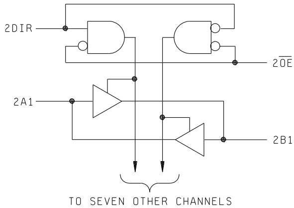
FIGURE 3. Logic diagram.
