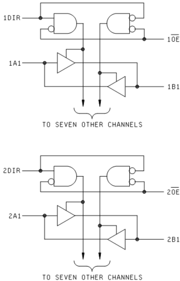
FIGURE 3. Logic diagram.
