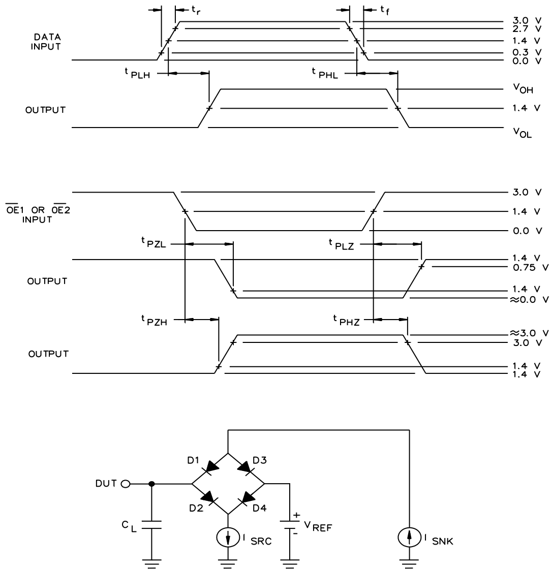
TEST CIRCUIT A OR EQUIVALENT
