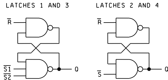
FIGURE 3. Logic diagram.
