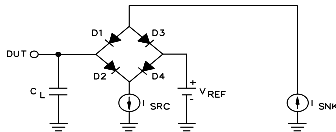
TEST CIRCUIT A OR EQUIVALENT
