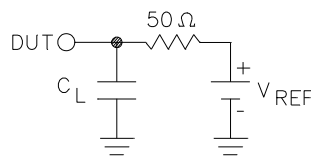
TEST CIRCUIT B OR EQUIVALENT
