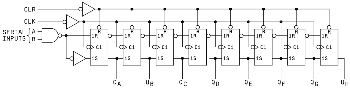
FIGURE 3. Logic diagram.
