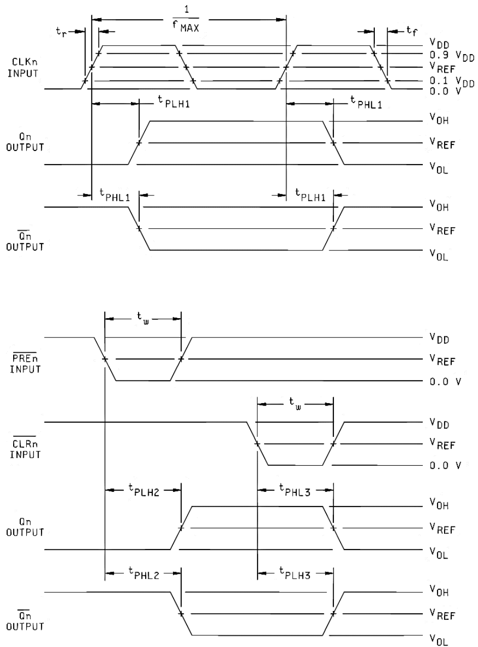
FIGURE 4. Switching waveforms and test circuits.
