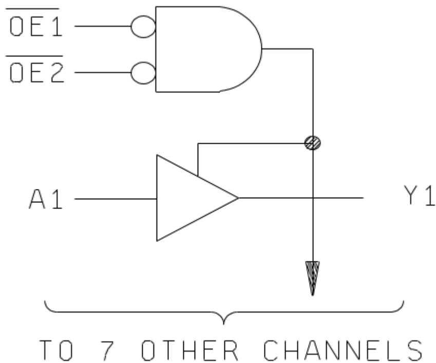
FIGURE 3. Logic diagram.
