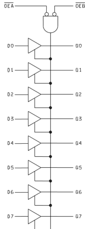
FIGURE 3. Logic diagram.
