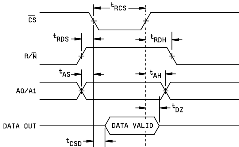
DATA OUTPUT (READ) TIMING
