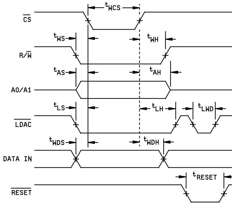
DATA WRITE (INPUT AND OUTPUT REGISTERS) TIMING
