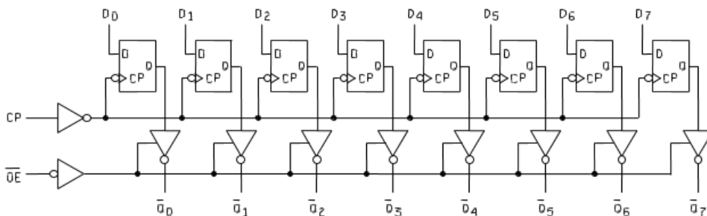
FIGURE 3. Logic diagram.
