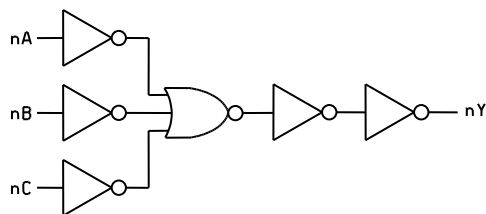
FIGURE 3. Logic diagram.
