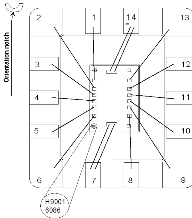
FIGURE A-1. Die bonding pad locations and electrical functions – Continued.
