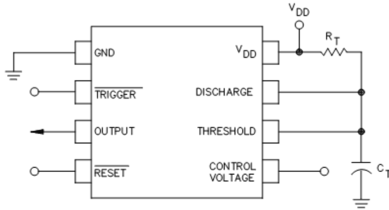
FIGURE 5. Monostable operation.
