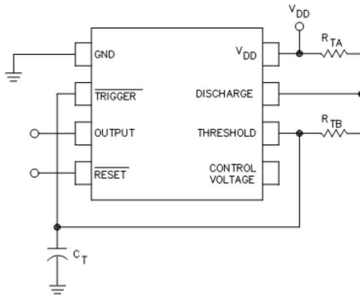
FIGURE 6. Astable operation.
