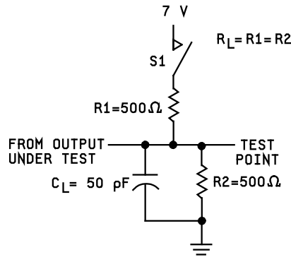
TEST CIRCUIT
