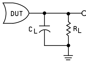
TEST CIRCUIT
