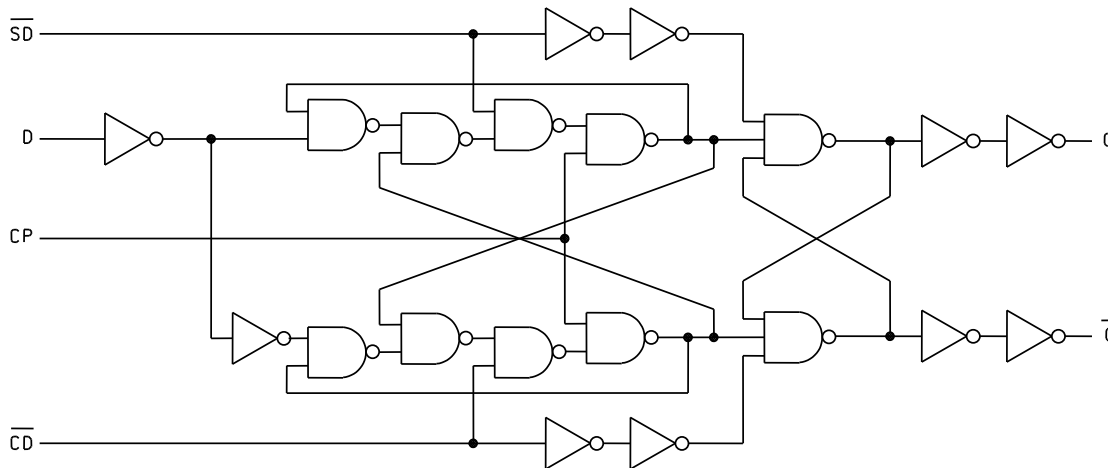
FIGURE 3. Logic diagram.
