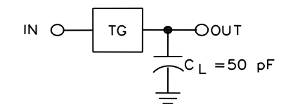
SWITCH IN TO SWITCH OUT PROPAGATION DELAY TEST CIRCUIT
