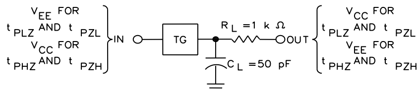
SWITCH ON/OFF PROPAGATION DELAY TEST CIRCUIT
