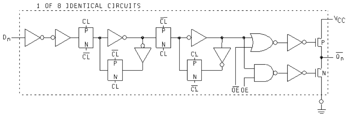
FIGURE 3. Logic diagram.
