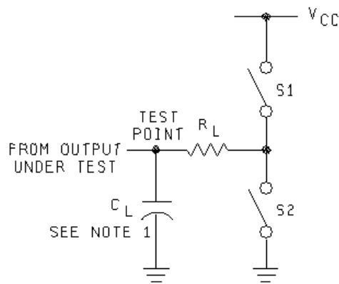
TEST CIRCUIT
