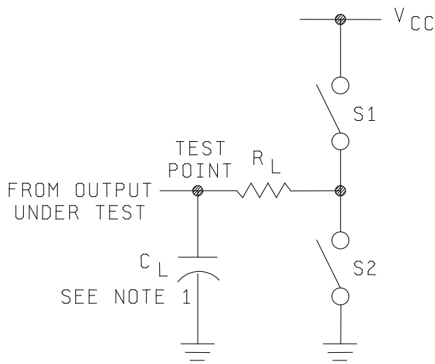
TEST CIRCUIT
