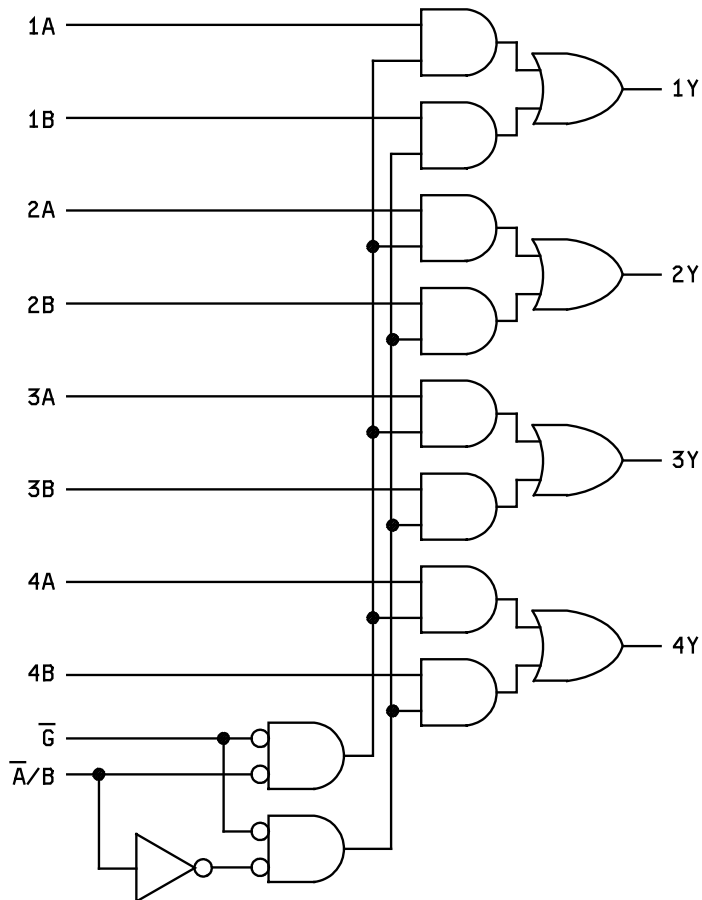
FIGURE 3. Logic diagram.
