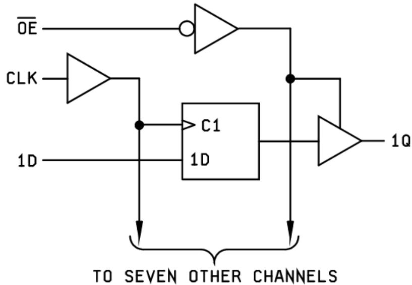
FIGURE 3. Logic diagram.
