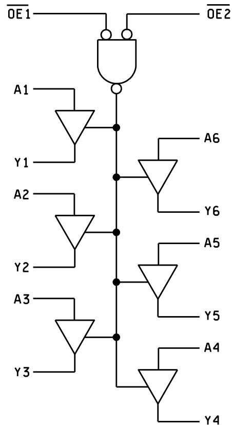
FIGURE 3. Logic diagram.
