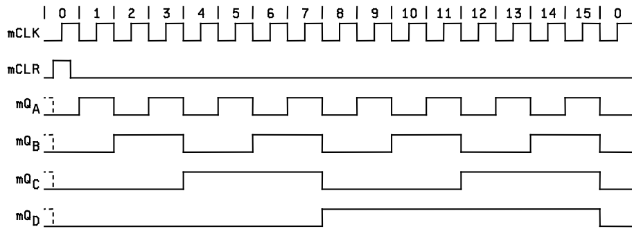
TIMING WAVEFORMS
