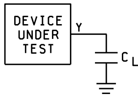
PROPAGATION DELAY TIME TEST CIRCUIT.
