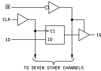
FIGURE 4. Logic diagram.
