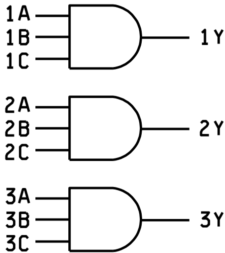
FIGURE 3. Logic diagram.
