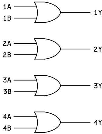
FIGURE 3. Logic diagram.
