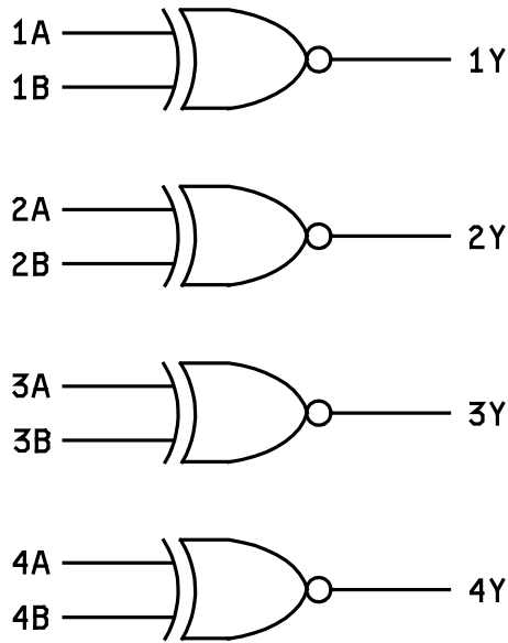
FIGURE 3. Logic diagram.
