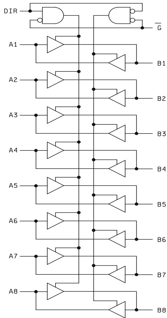
FIGURE 3. Logic diagram.
