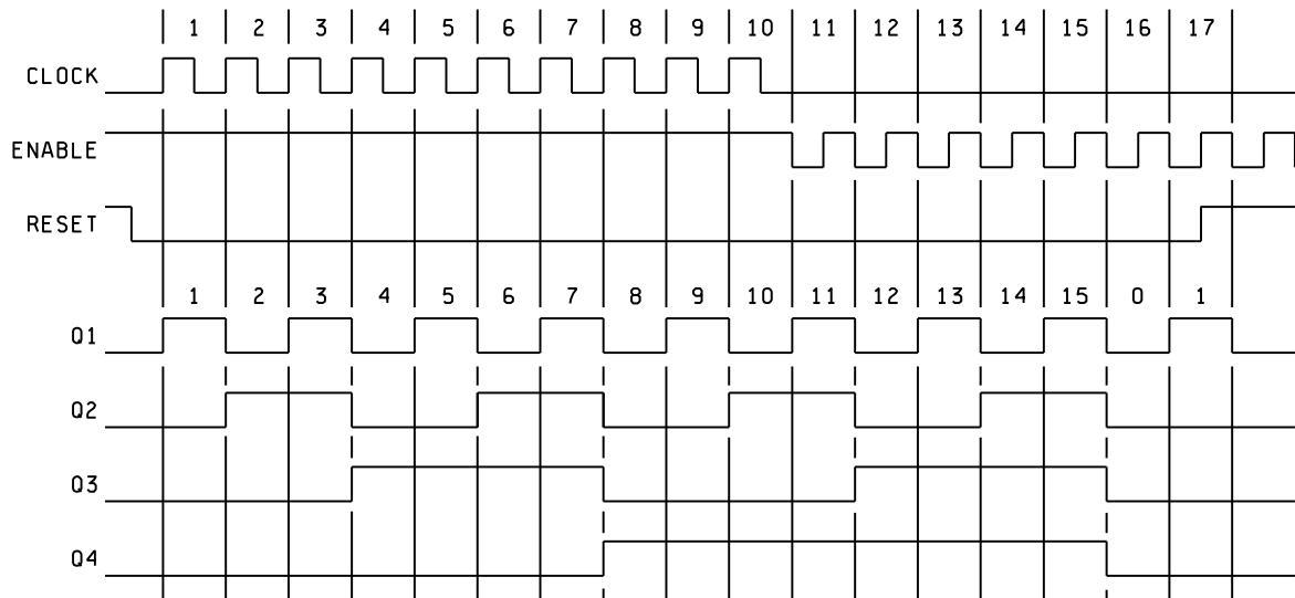
FIGURE 4. Counting sequence.
