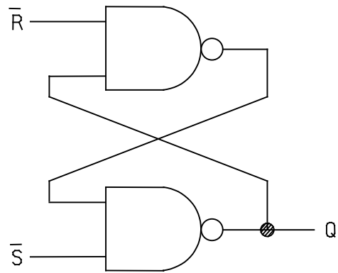
LATCHES 2 AND 4
