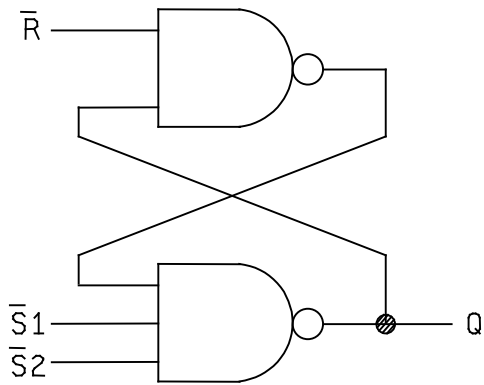
LATCHES 1 AND 3
