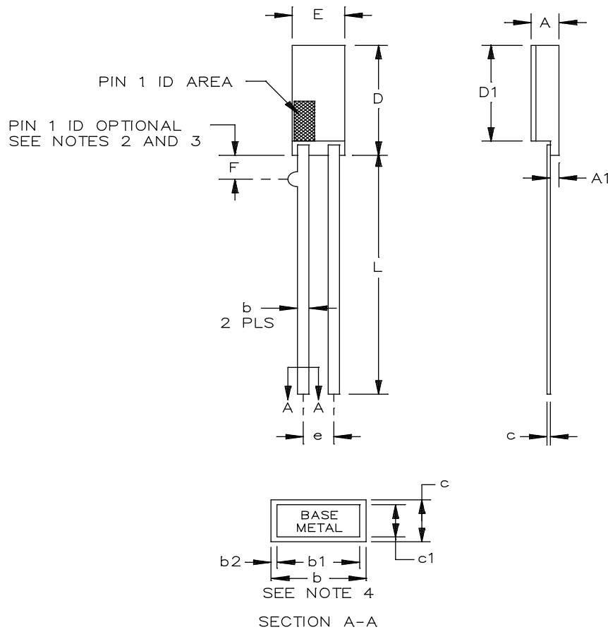
FIGURE 1. Case outline.
