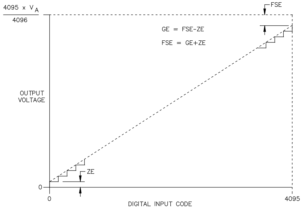
FIGURE 2. Input / output transfer characteristic.
