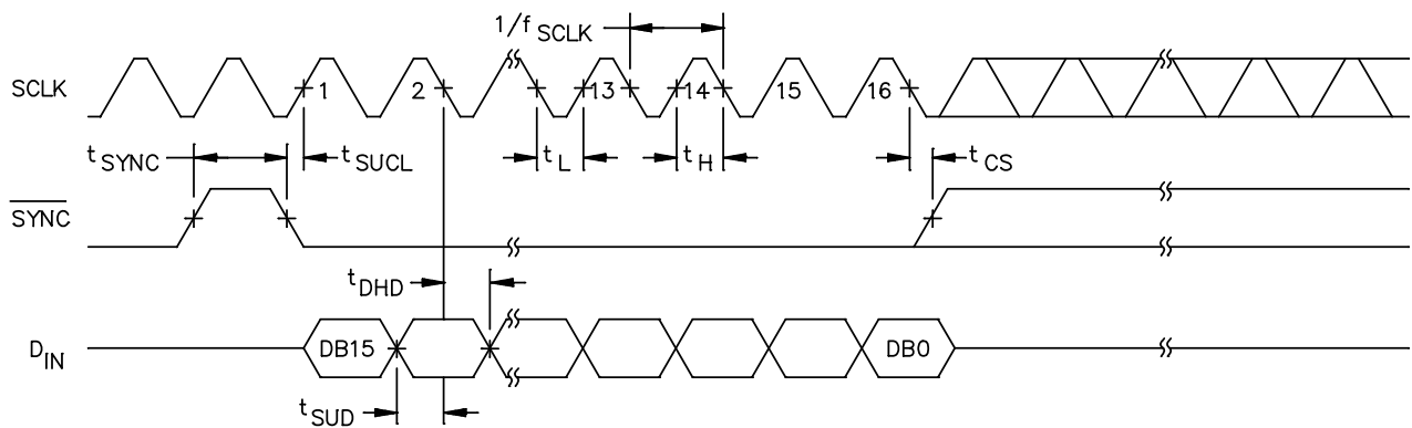
FIGURE 3. Timing waveforms.
